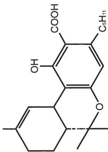
delta 9-THCA
