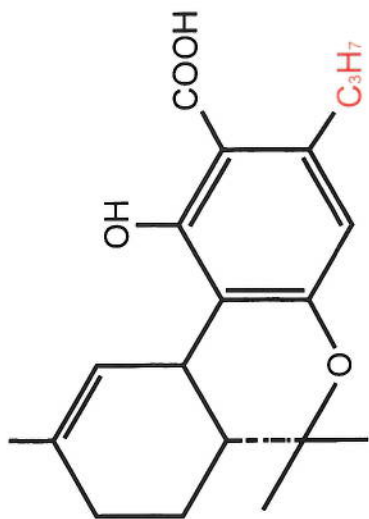
delta 9-THCVA
