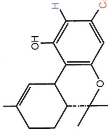
delta 9-THCV
