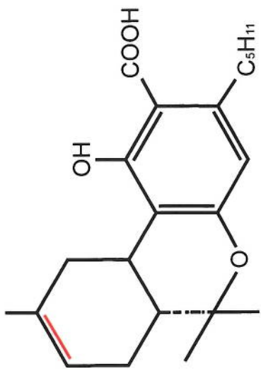
delta 8-THCA
